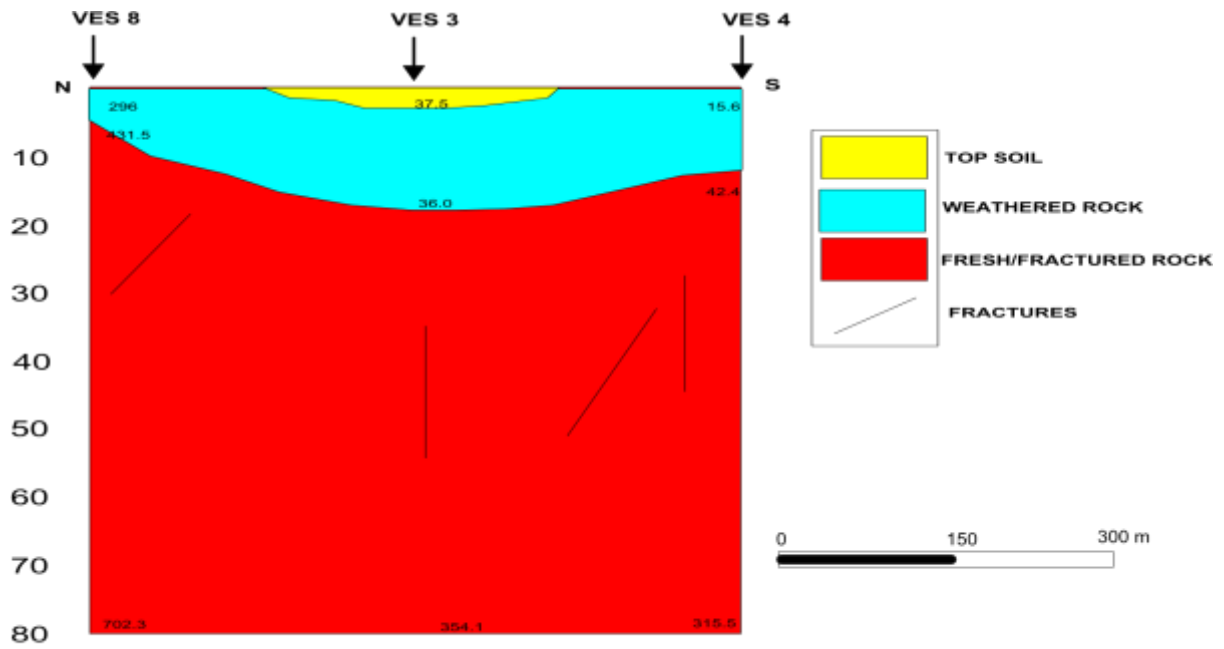
Fig. 10. Geoelectric Section for Profile 2.
