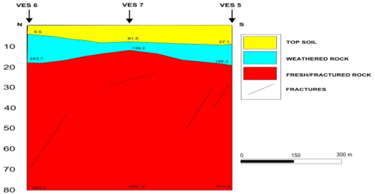
Fig. 11. Geoelectric Section for Profile 3.
