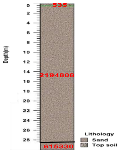
Figure 3: Lithology of VES 1
