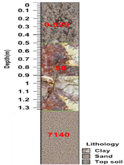
Figure 6: Lithology of VES 3
