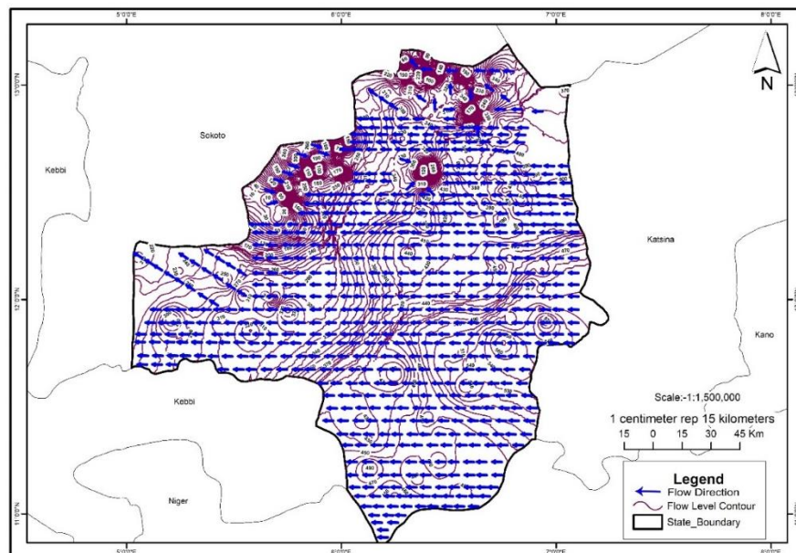
Figure 16: Groundwater Flow Pattern of the Study Area
