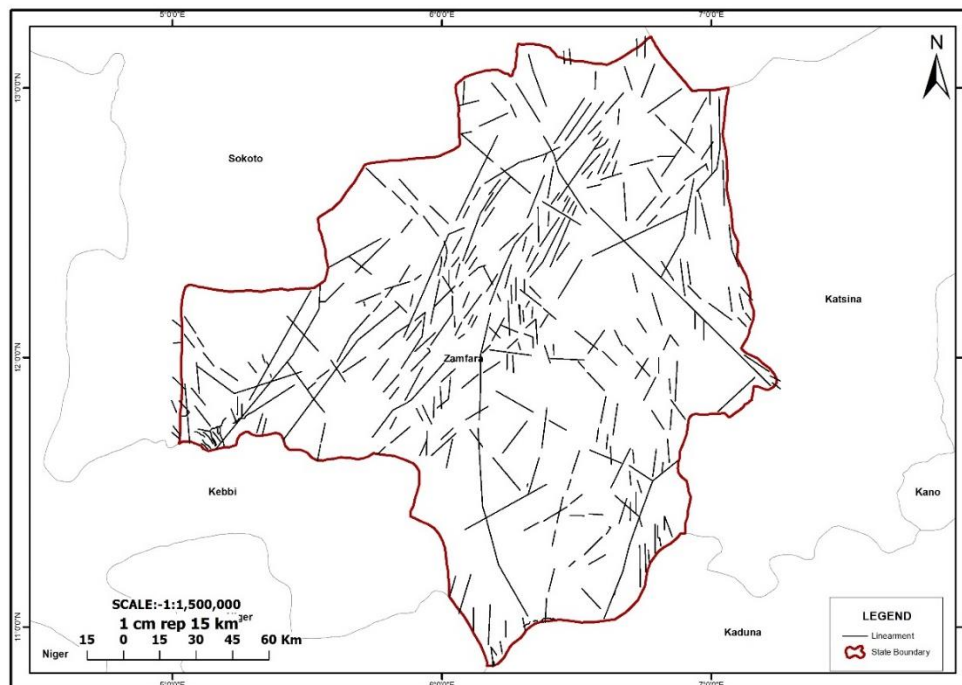
Figure 4: Lineament map of the study area
