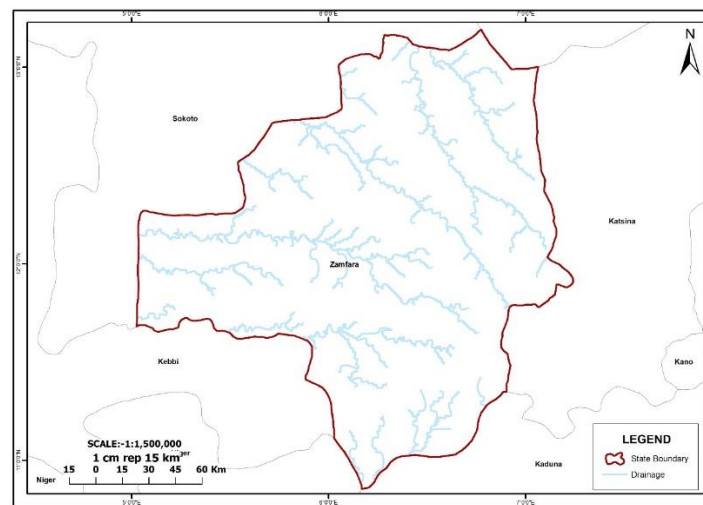
Figure 8: Drainage map of the study area
