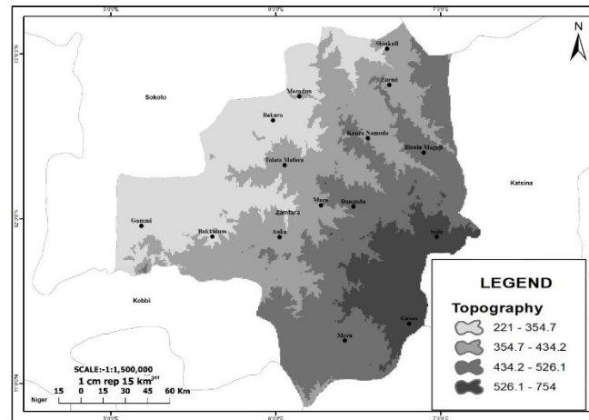
Figure 6: Geomorphological map of the study area
