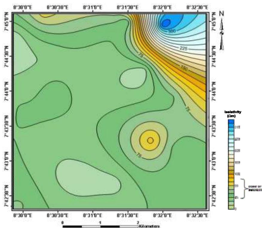
Figure 10: Iso-resistivity contour at a depth of 50
