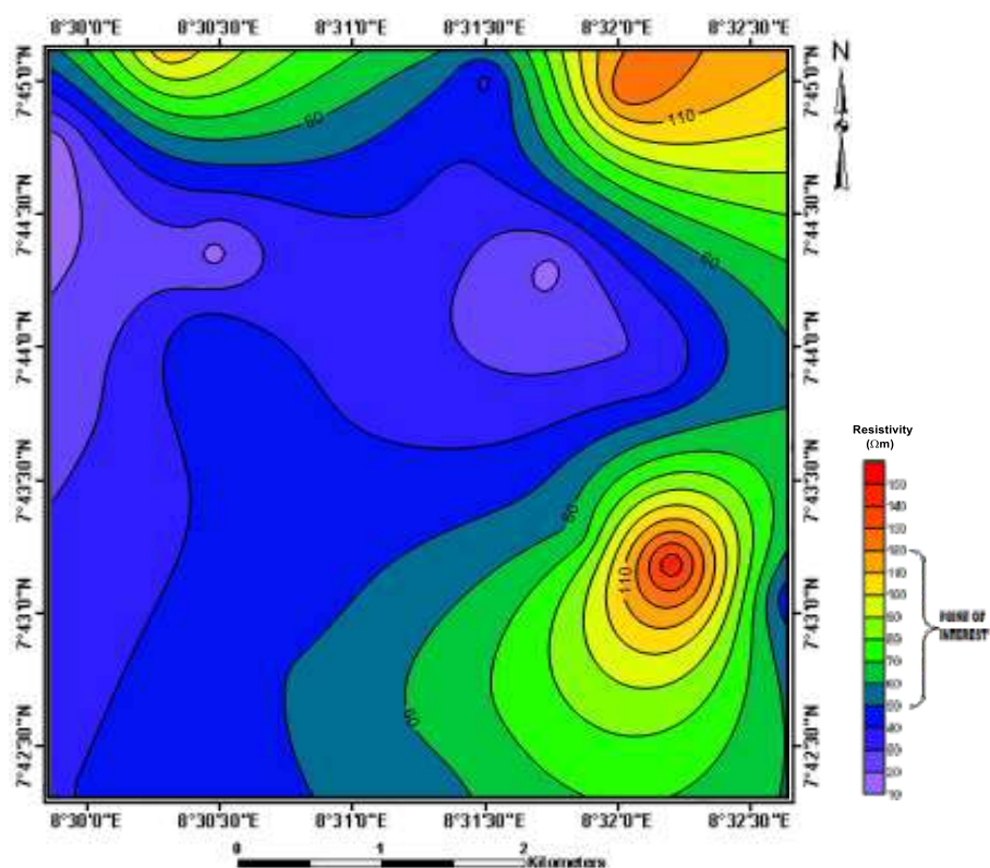
Figure 9: Iso-resistivity contour at a depth of 30m
