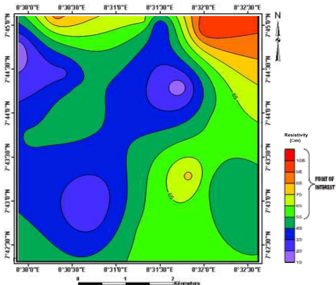
Figure 8: Isoresistivity contour at a depth of 20m
