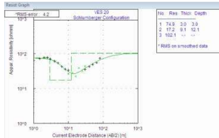
Figure 7: VES 20 Geo-Electric curve
