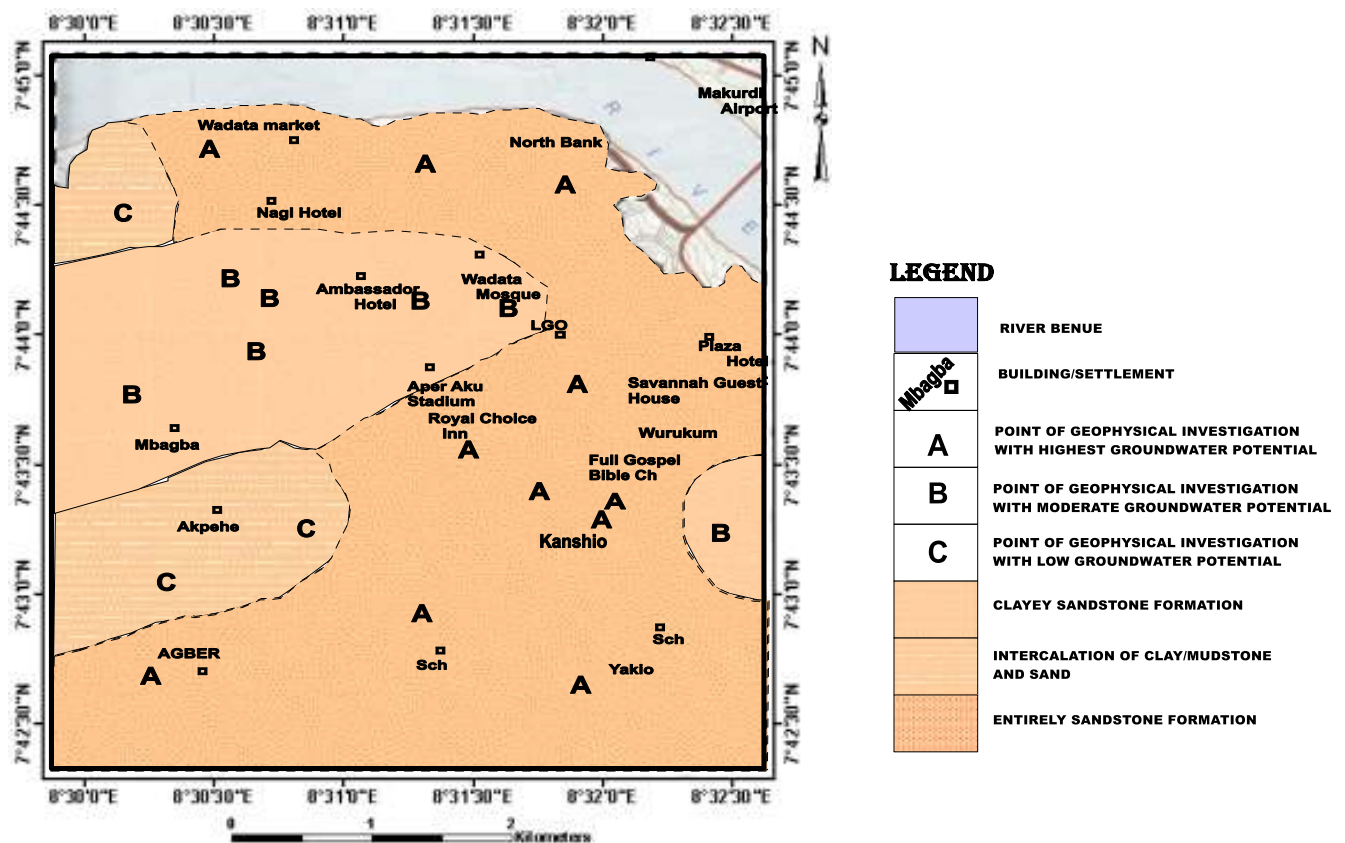
Figure 11: Groundwater potential map of the study area
