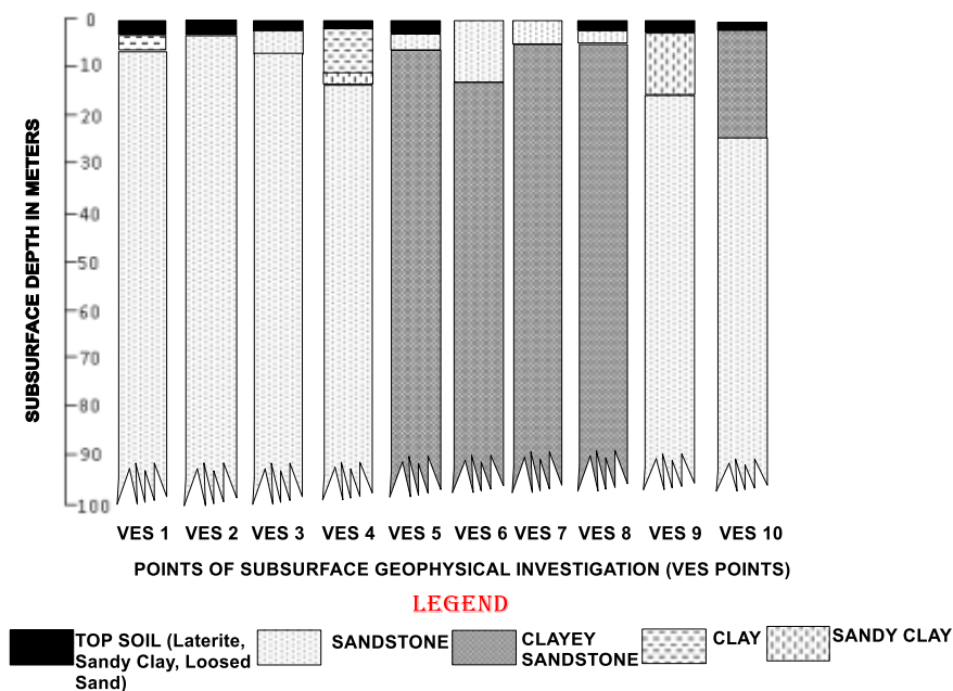
Figure 4: Geoelectric profiles for VES locations 1-10
