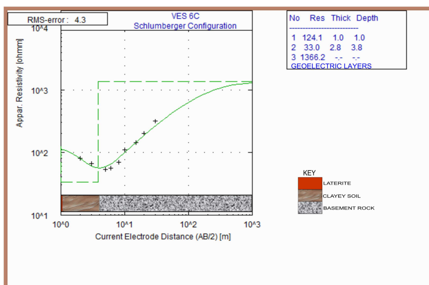
Fig.4b: HA Sounding Curve
