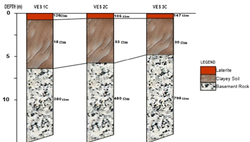
Fig.5a Geoelectric section 1C
