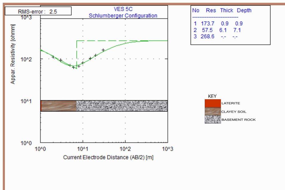
Fig. 4a: H Sounding Curve
