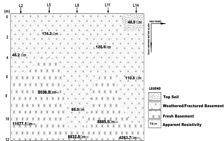
Figure 7: Geoelectric Section for Profile 1.
