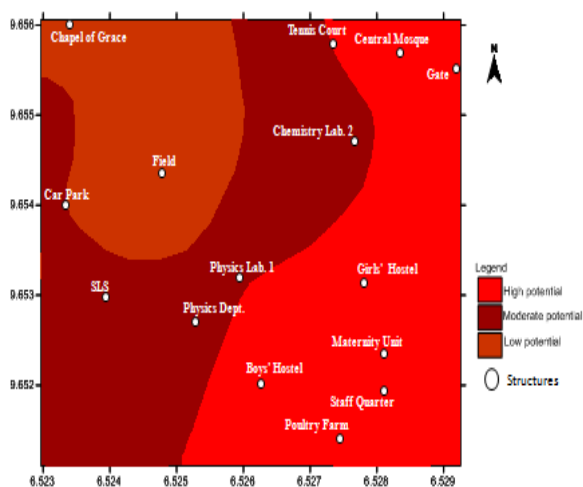
Figure 10: Groundwater Potential Map.
