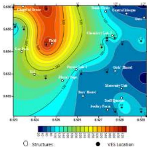
Figure 8: Iso – Resistivity at 10m.
