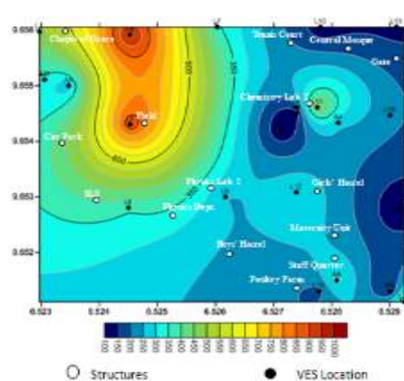
Figure 9: Iso – Resistivity at 30m.
