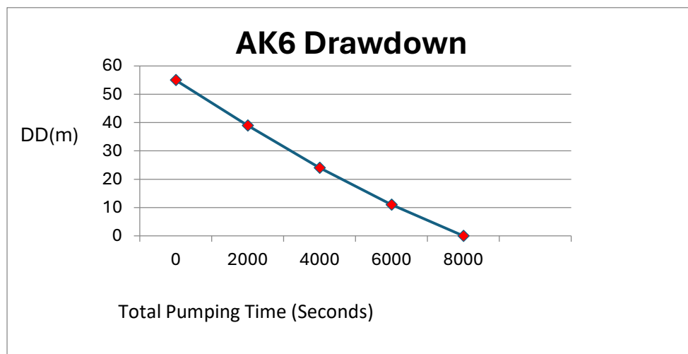
Figure 3: Detail of drawdown graph at AK6 borehole
