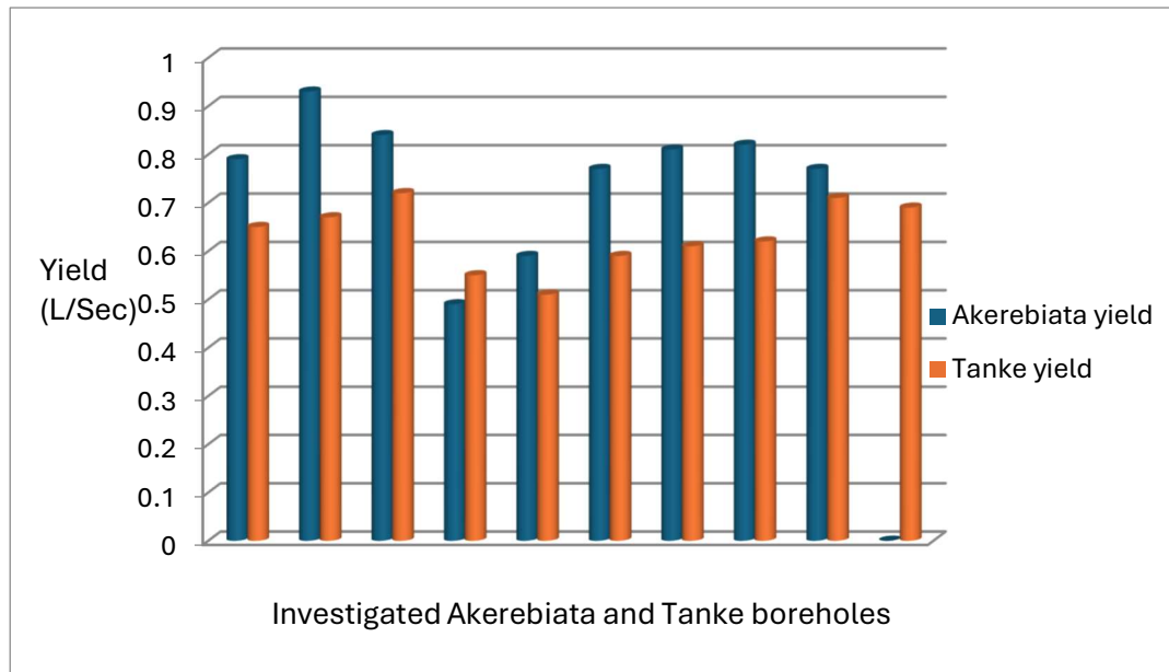
Figure 6: Comparative yield of Akerebiata and Tanke wells
