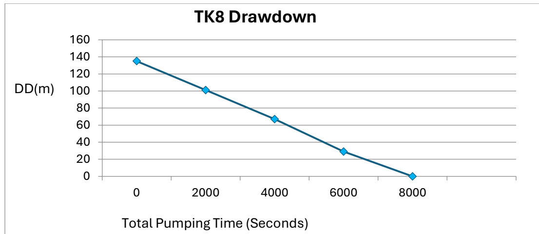
Figure 5: Drawdown graph of TK8 Borehole
