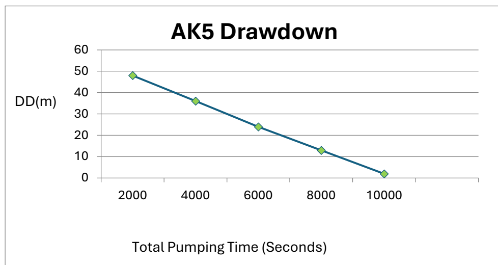
Figure 2: Detail of drawdown graph of AK5 borehole
